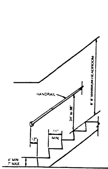
HANDRAIL AND STAIR DETAIL
