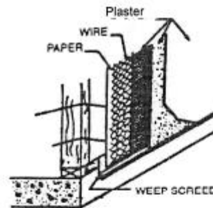
TERMINATION OF EXTERIOR PLASTER AT ON-GRADE CONCRETE FLOOR FOR STUD WALLS
